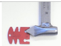
FOREPUNCH GAUGE
